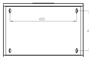
REAR VIEW
