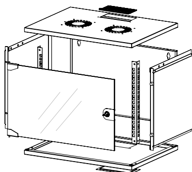
EXPLODED VIEW
